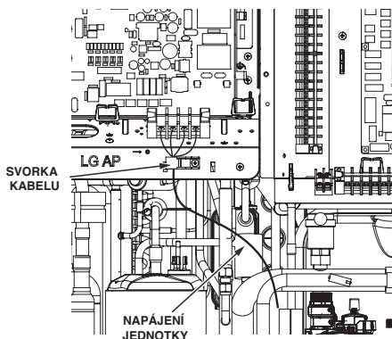
UN36A (5, 7, 9 kW)
